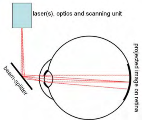
Fig 2.2: Simplified diagram of a retinal Display.
